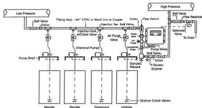
TYPICAL LAYOUT: COOLING WATER TREATMENT PROGRAM & TOWER CONTROL AND PRODUCT FEED EQUIPMENT
